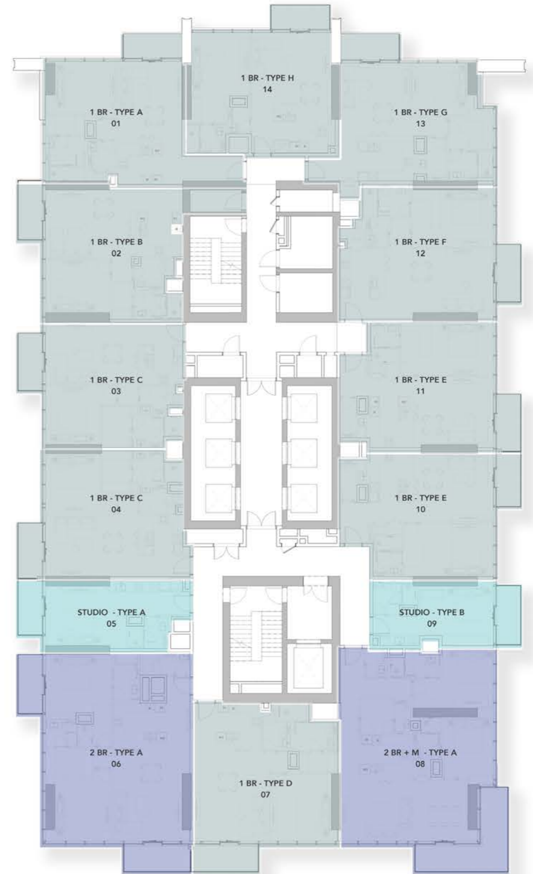
8TH-20TH TYPICAL FLOOR PLAN
